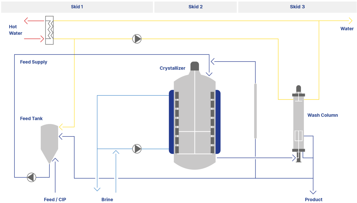
Image 1: Freeze concentration process. Image: GEA
