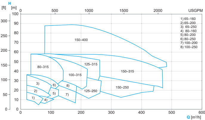
GEAHILGE MAXA PERFORMANCE CURVE 60 HZ – 4-POLE
