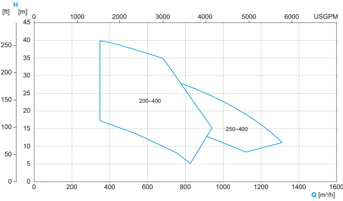
GEAILGE MAXA PERFORMANCE CURVE 60 Z – 6-POLE
