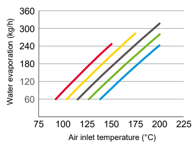
VSD-80 co-current atomization
