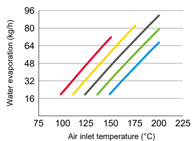
VSD-50 co-current atomization
