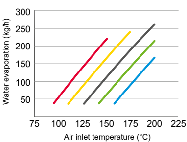
VFSD-80 co-current atomization
