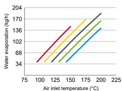
VSD-50 co-current atomization
