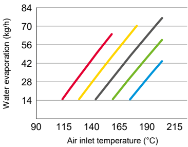
VFSD-50 co-current atomization
